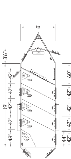
TRADITION BP 8' wide four horse bumper pull
