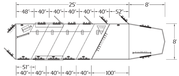
TRADITION 8' wide five horse gooseneck with mangers
