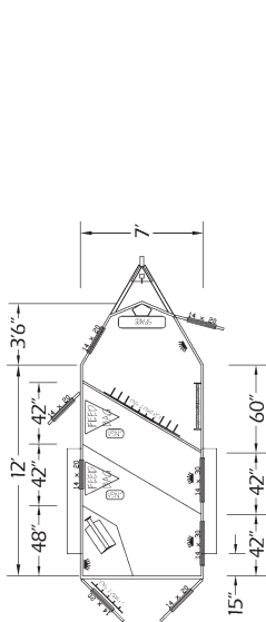
TRADITION BP 7' wide two horse bumper pull
