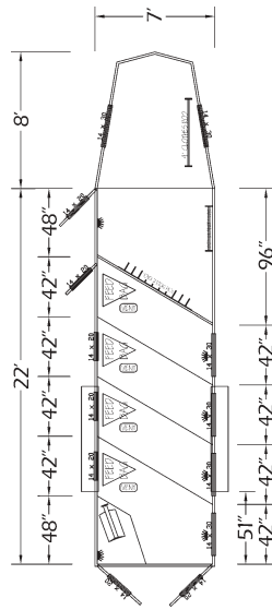
TRADITION 7' wide four horse gooseneck
