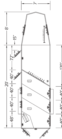
LEGEND HERITAGE III Three horse gooseneck with 6' dressing room
