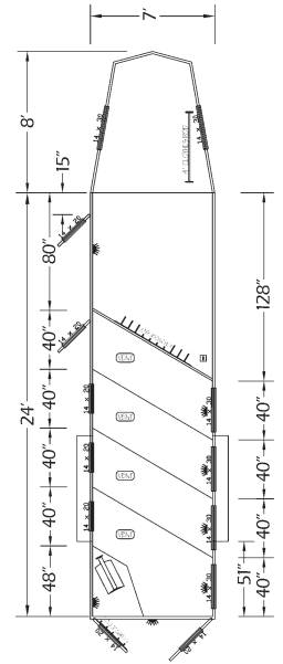
LEGEND HERITAGE III Four horse gooseneck with 6' dressing room
