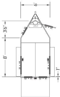
LEGEND CONTENDER I 6' wide two horse bumper pull
