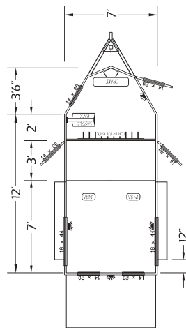
LEGEND CONTENDER II 7' wide bumper pull with dressing room
