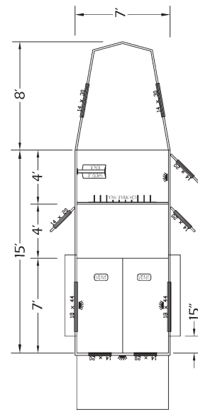
LEGEND CONTENDER III Gooseneck with dressing room
