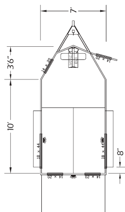
LEGEND CONTENDER I.5 7' wide two horse bumper pull
