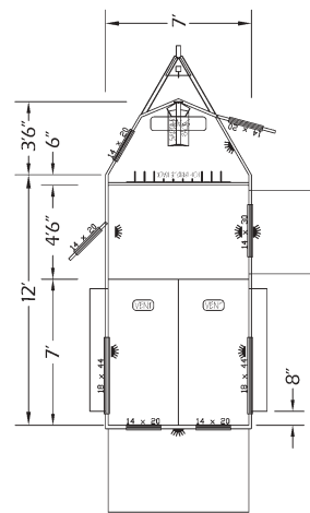
LEGEND CONTENDER II 7' wide bumper pull with dressing room and side ramp
