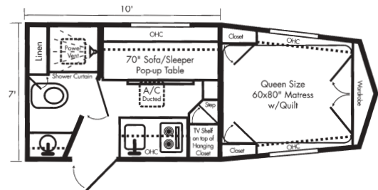
FREEDOM II Sample interior
