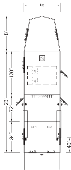
FREEDOM II 8' wide two horse straight load gooseneck
