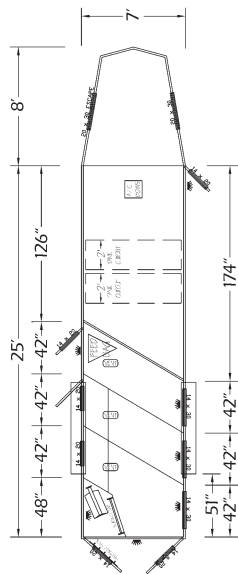
FREEDOM I 7' wide three horse slant load gooseneck with mangers
