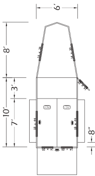
COMPETITOR Two horse gooseneck
