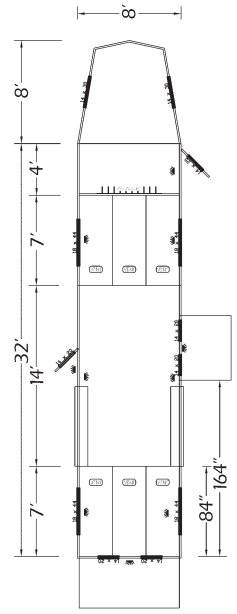
COMPETITOR IV Six horse gooseneck with dressing room
