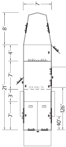
COMPETITOR I Two horse gooseneck with dressing room
