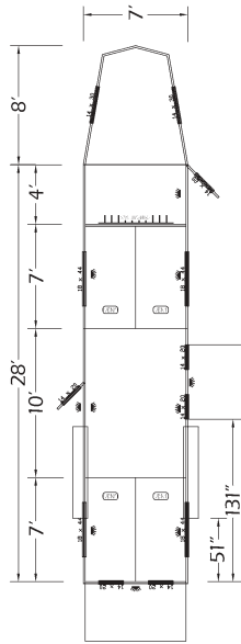
COMPETITOR II Four horse gooseneck with dressing room
